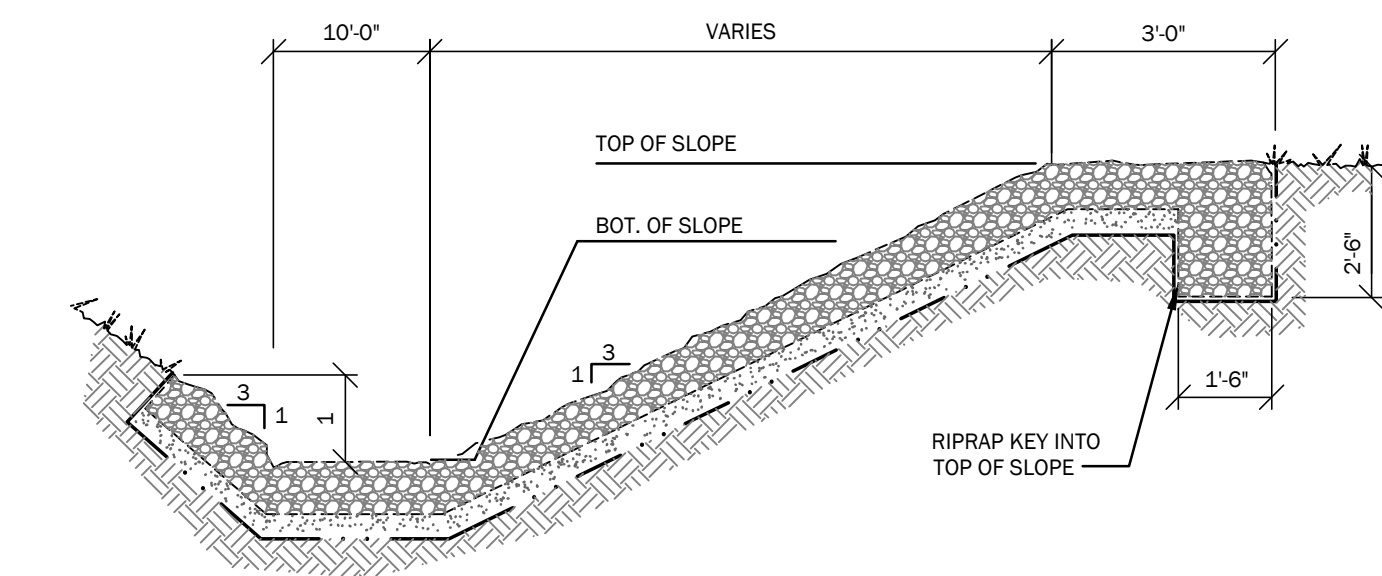
PROFILE @ CENTERLINE
