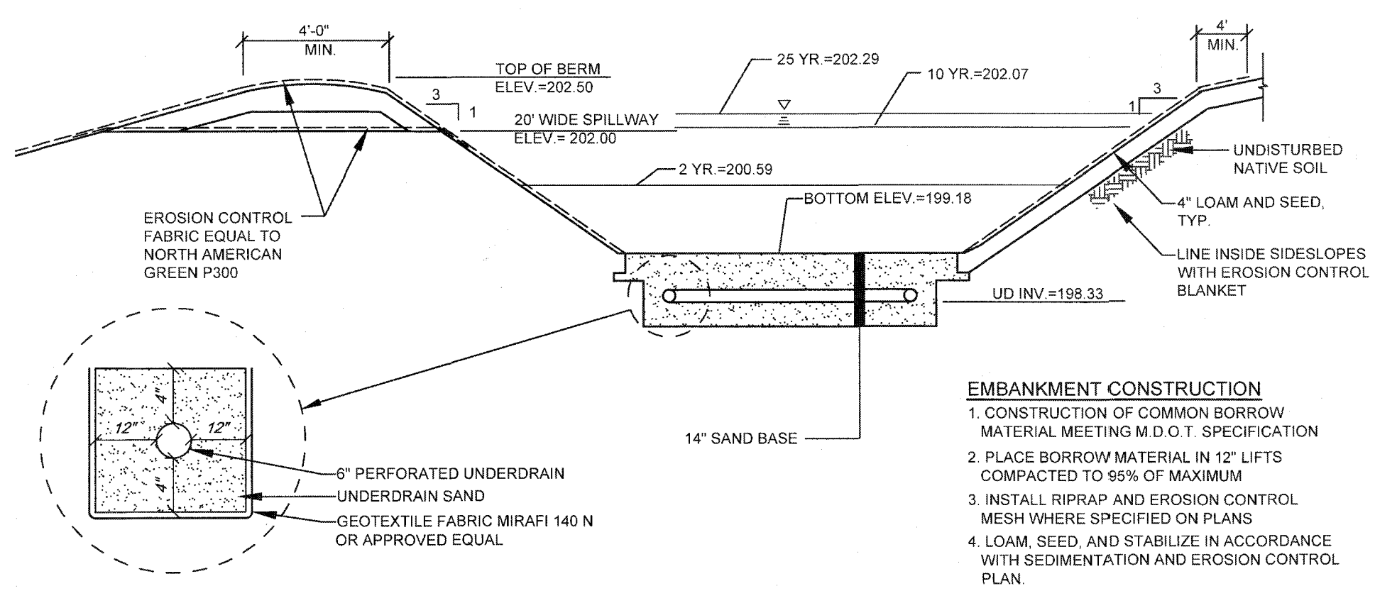
DETENTION BASIN 1 SECTION NOT TO SCALE
