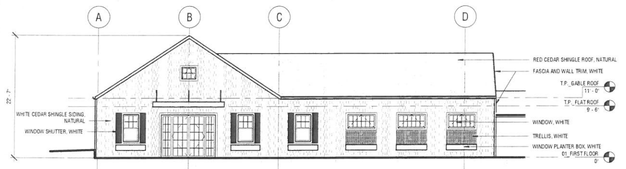
6 SOUTH ELEVATION 1/8" = 1'-0"
