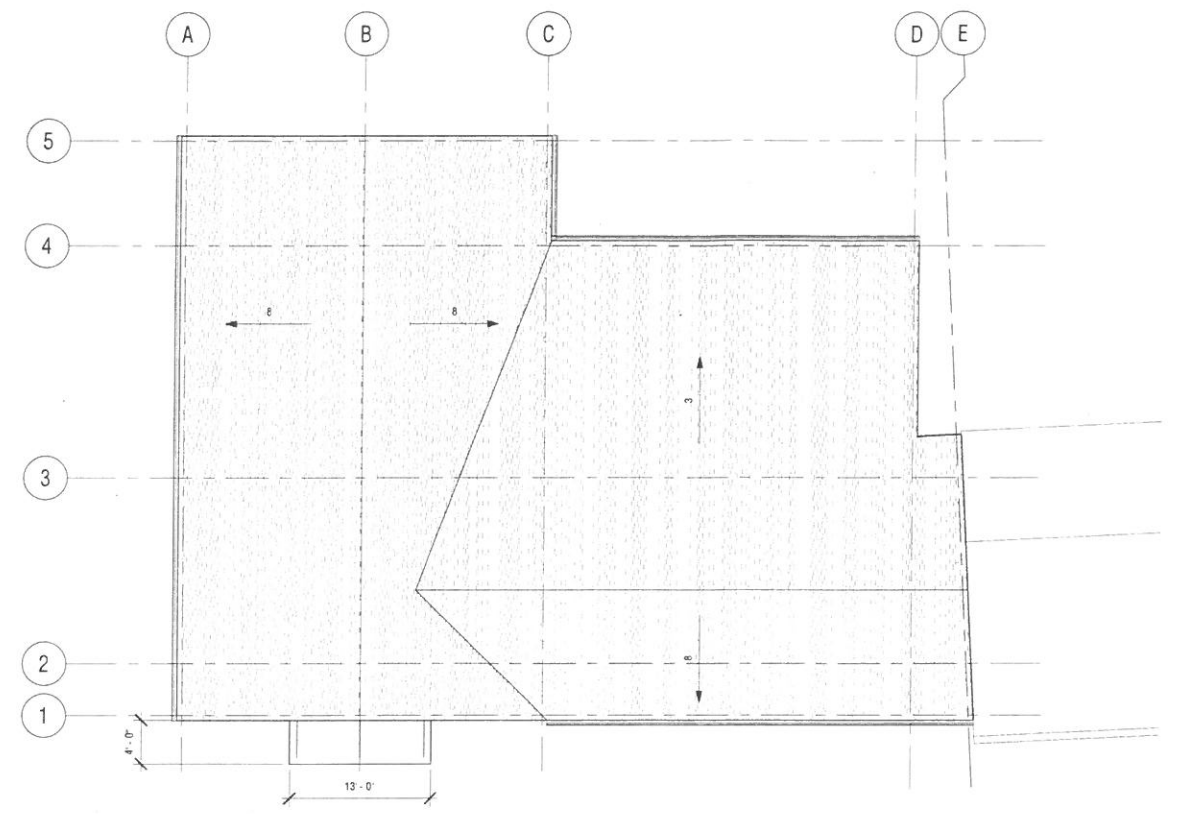
2 02 ROOF PLAN PB 1/8" = 1'-0"
