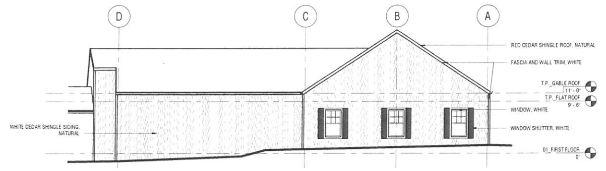
5 NORTH ELEVATION 1/8" = 1'-0"
