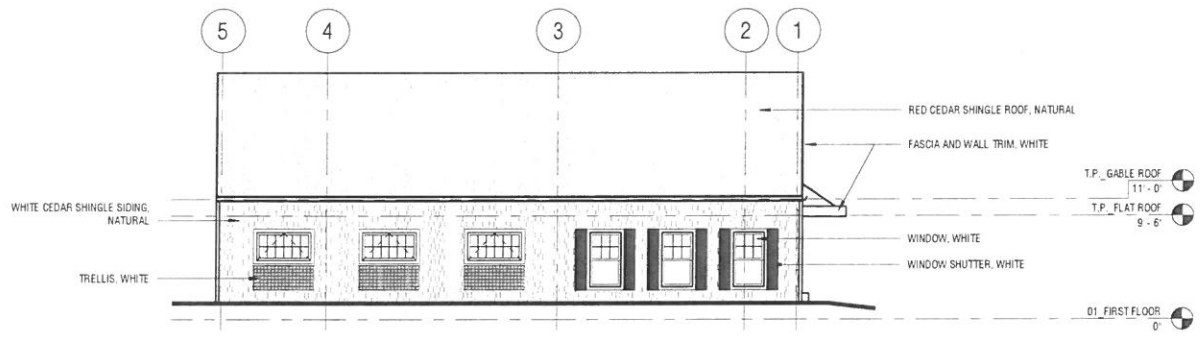
4 WEST ELEVATION 1/8" = 1'-0"
