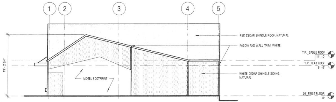
3 EAST ELEVATION 1/8" = 1'-0"
