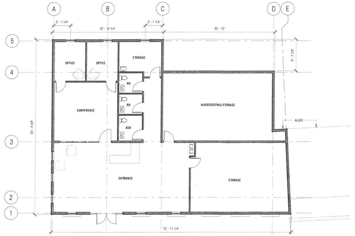
1 01 FIRST FLOOR PLAN PB 1/8" = 1'-0"
